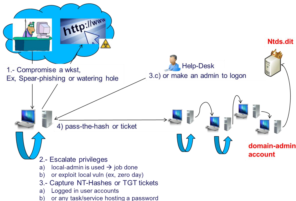
Figure 1 - Typical lateral movements in APTs
